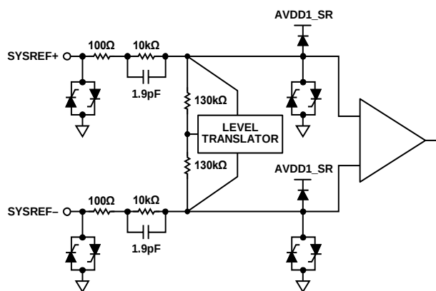
Figure 59. SYSREF± Inputs
