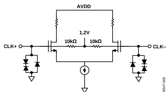
Figure 9. Equivalent Clock Input Circuit
