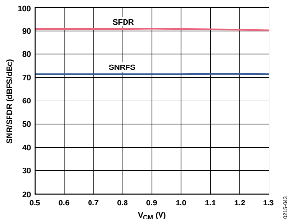
Figure 44. SNR/SFDR vs. Common-Mode Voltage, f_{IN} = 9.7 \text{ MHz} , f_{SAMPLE} = 80 \text{ MSPS}
