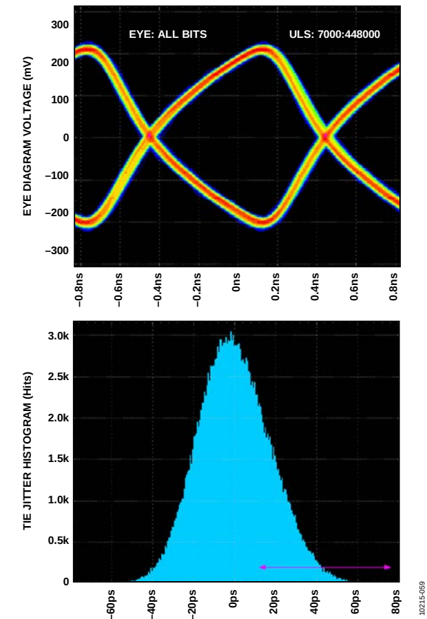
Figure 60. Data Eye for LVDS Outputs in ANSI-644 Mode with Trace Lengths Greater Than 24 Inches on Standard FR-4, External 100 \Omega Far Termination Only
