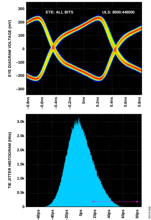
Figure 59. Data Eye for LVDS Outputs in ANSI-644 Mode with Trace Lengths of Less Than 24 Inches on Standard FR-4, External 100 \Omega Far-End Termination Only
