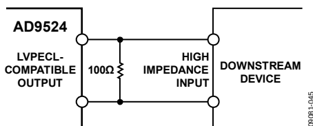
Figure 18. DC-Coupled LVPECL Output Driver
