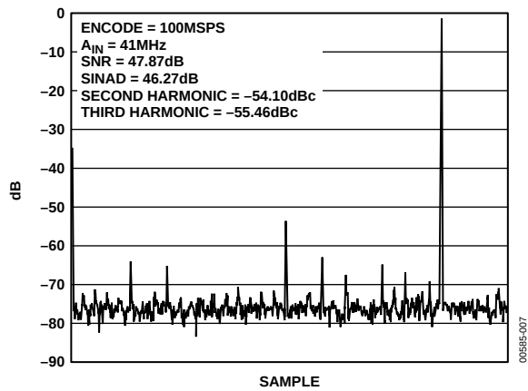
Figure 7. Spectrum: f_s = 100 MSPS, f_{IN} = 41 MHz, Single-Ended Input
