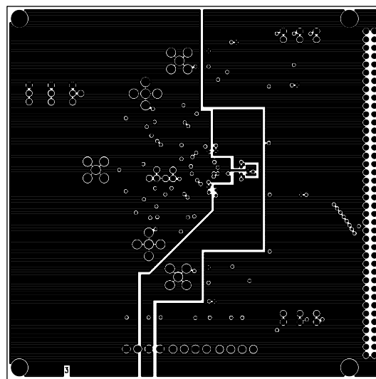
Figure 31. Split Power Plane
