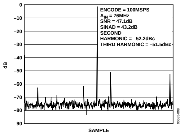
Figure 8. Spectrum: f_s = 100 MSPS, f_{IN} = 76 MHz, Single-Ended Input
