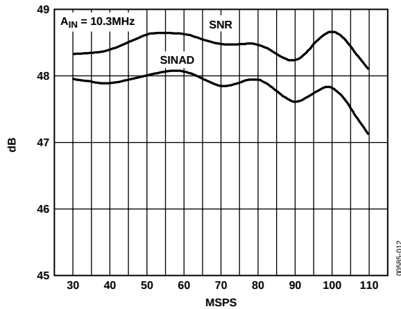
Figure 12. SINAD/SNR vs. Encode Rate
