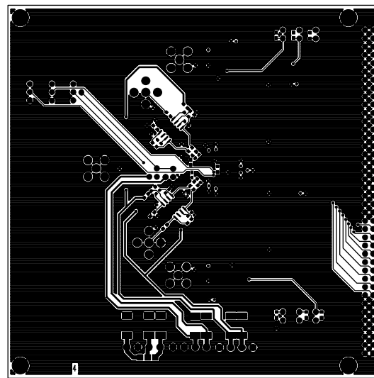
Figure 32. Bottom Routing
