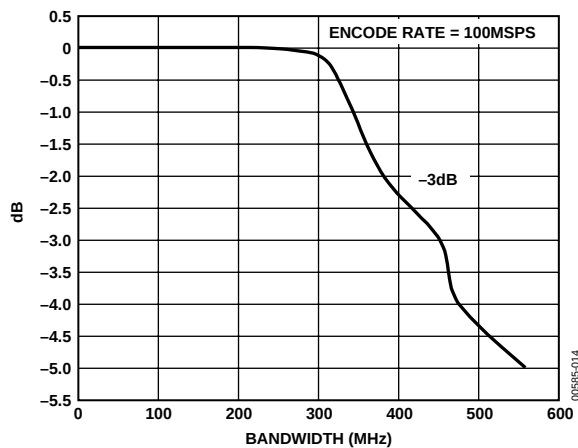
Figure 14. ADC Frequency Response: f_s = 100 MSPS
