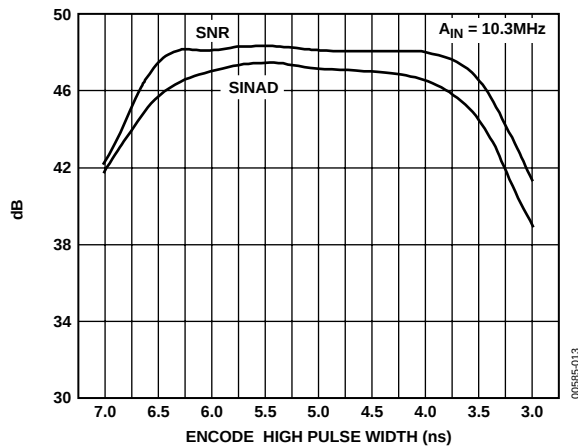
Figure 13. SINAD/SNR vs. Encode Pulse Width High
