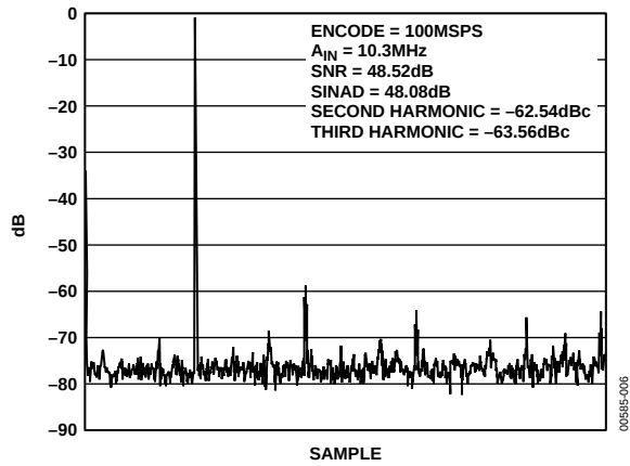
Figure 6. Spectrum: f_s = 100 MSPS, f_{IN} = 10 MHz, Single-Ended Input
