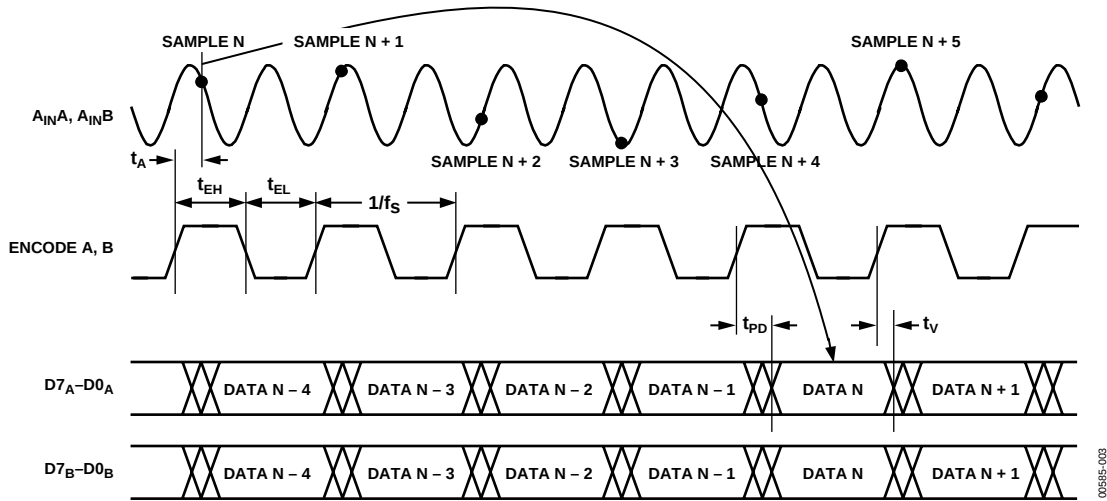
Figure 2. Normal Operation, Same Clock ( S1 = 1, S2 = 0 ) Channel Timing
