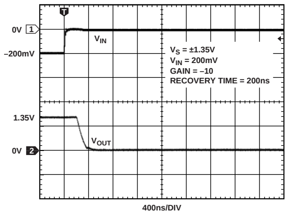
Figure 44. Positive Overload Recovery Time
