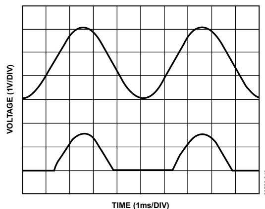
Figure 50. Half-Wave Rectifier Signal (OUT A in Figure 49)
