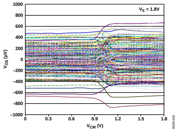
Figure 26. Input Offset Voltage vs. Input Common-Mode Voltage
