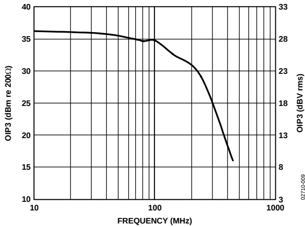
Figure 9. OIP3 vs. Frequency for V_{\text{GAIN}} = 500 \text{ mV}
