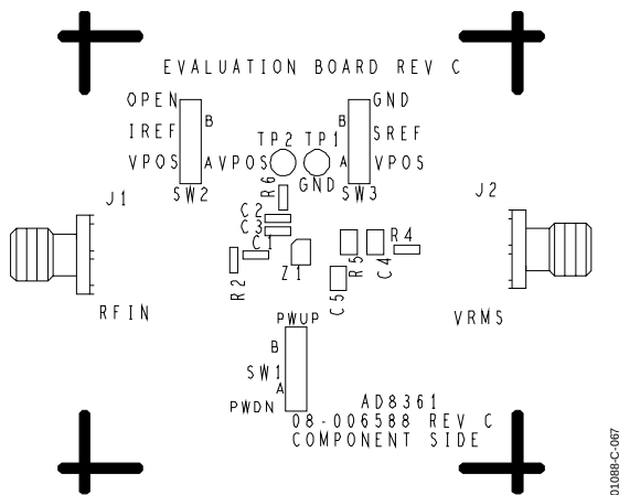
Figure 61. Layout of Component Side, MSOP
