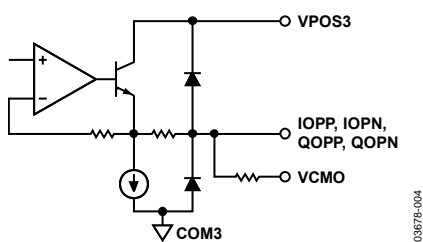
Figure 4. Circuit B
