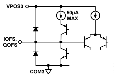
Figure 8. Circuit F
