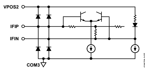
Figure 7. Circuit E
