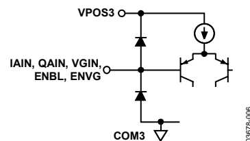
Figure 6. Circuit D
