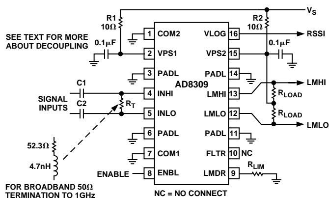
Figure 30. Basic Connections
