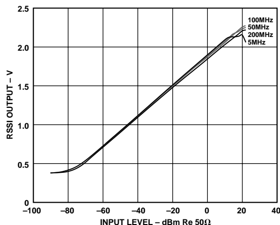
Figure 31. RSSI Output vs. Input Level at T A = +25°C, for Frequencies of 5 MHz, 50 MHz, 100 MHz and 200 MHz
