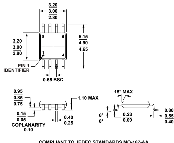
Figure 37. 8-Lead Mini Small Outline Package [MSOP] (RM-8)
