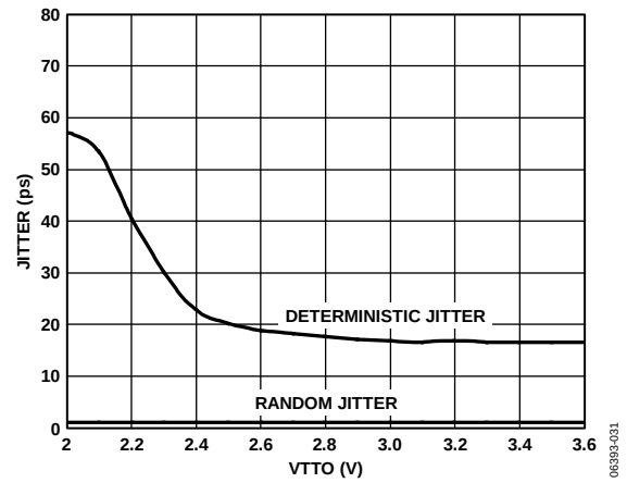
Figure 26. Jitter vs. Output Termination Voltage
