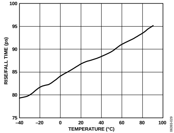
Figure 27. Rise/Fall Time vs. Temperature
