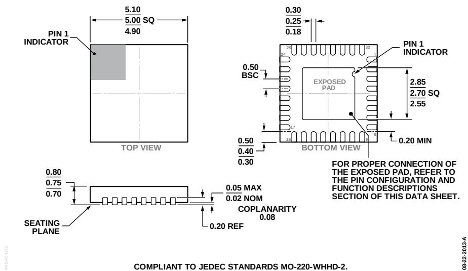
Figure 41. 32-Lead Lead Frame Chip Scale Package [LFCSP_WQ] 5 mm x 5 mm Body, Very Very Thin Quad (CP-32-21) Dimensions shown in millimeters
