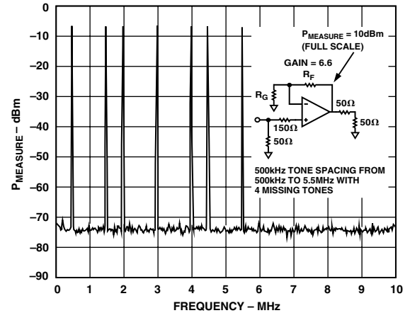
Figure 12. Multitone Distortion; R_L = 100\ \Omega
