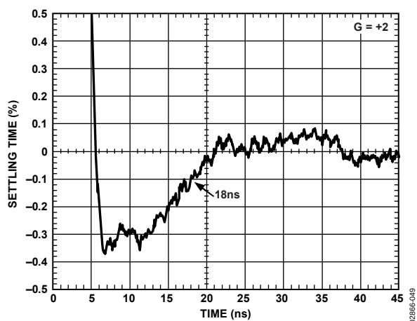
Figure 49. 0.1% Settling Time, 2\text{ V} Step
