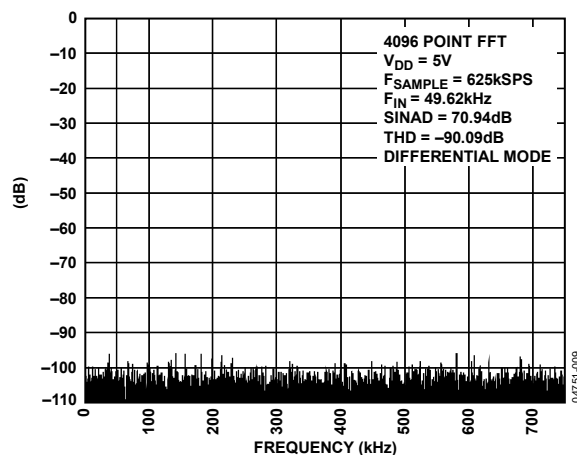
Figure 7. AD7938-6 FFT at V_{DD} = 5\text{V}
