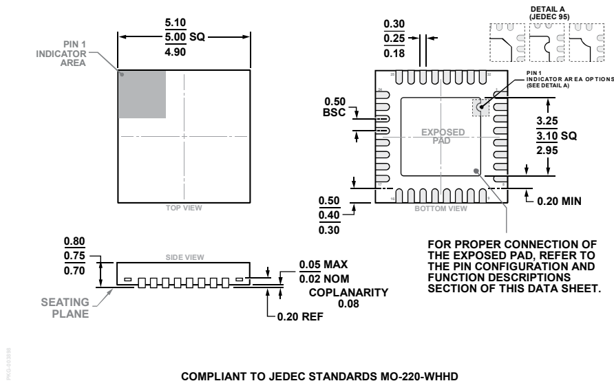
Figure 47. 32-Lead Lead Frame Chip Scale Package [LFCSP] 5 mm × 5 mm Body and 0.75 mm Package Height (CP-32-7) Dimensions shown in millimeters
