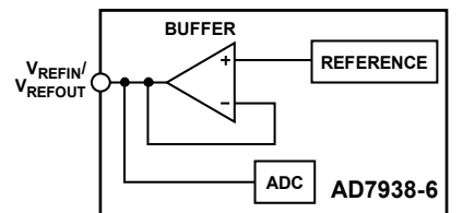
Figure 34. Internal Reference Circuit Block Diagram
