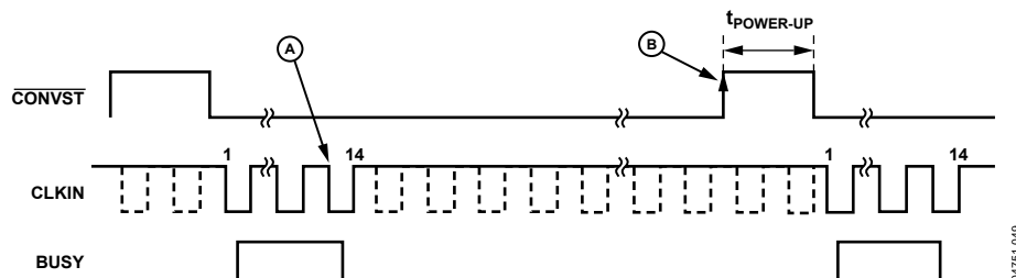
Figure 40. Autoshutdown/Autostandby Mode
