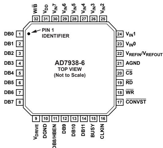
Figure 3. Pin Configuration (SU-32-2)
