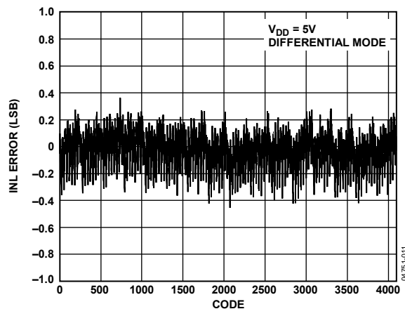
Figure 9. AD7938-6 Typical INL at V_{DD} = 5\text{V}
