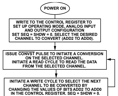
Figure 31. Traditional Multichannel Operation Flow Chart
