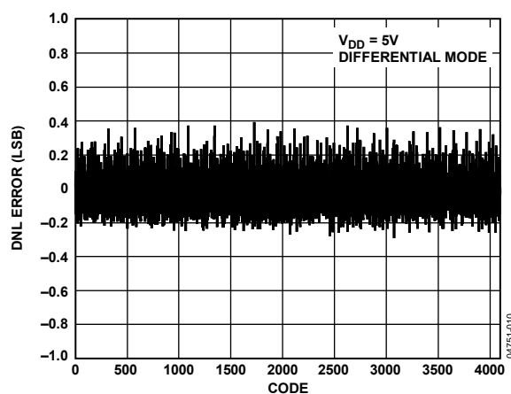
Figure 8. AD7938-6 Typical DNL at V_{DD} = 5\text{V}
