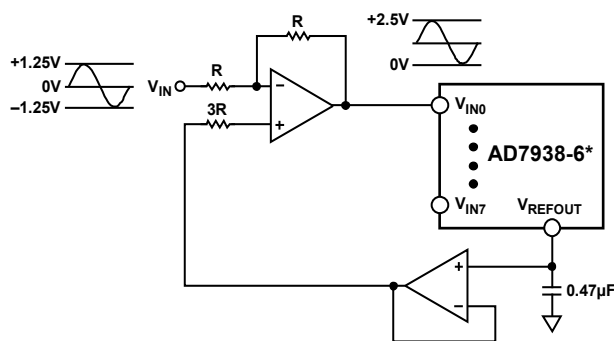
Figure 24. Single-Ended Mode Connection Diagram
