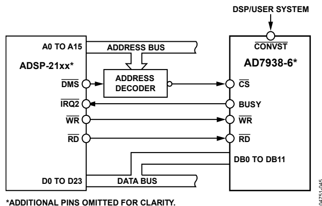
Figure 43. Interfacing to the ADSP-21xx
