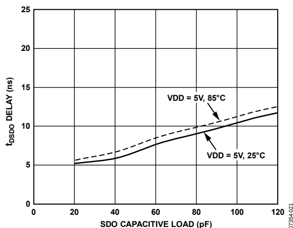
Figure 25. t_{DSO} Delay vs. SDO Capacitive Load and Supply
