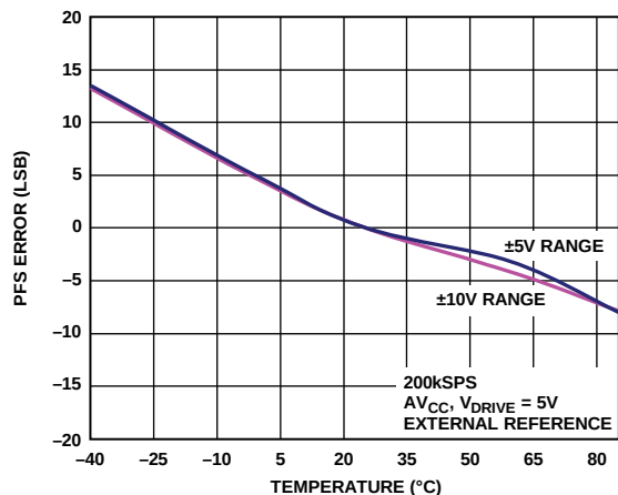
Figure 19. PFS Error vs. Temperature
