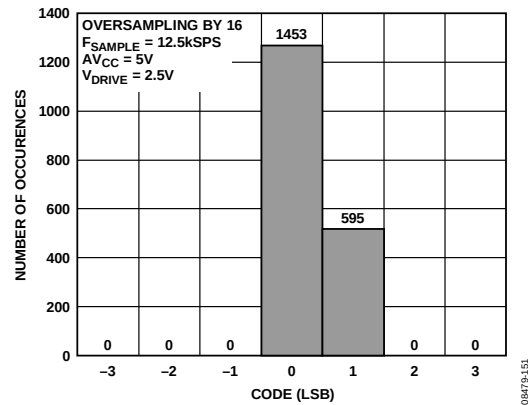
Figure 53. Histogram of Codes—OS × 16 (Two Codes)
