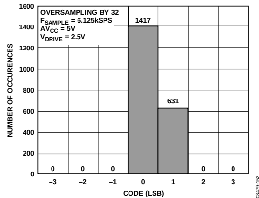
Figure 54. Histogram of Codes—OS × 32 (Two Codes)
