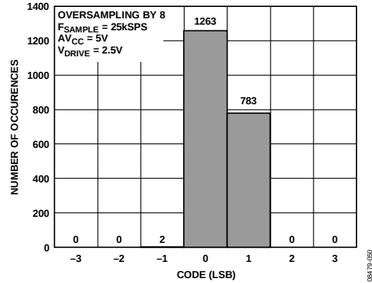
Figure 52. Histogram of Codes—OS × 8 (Three Codes)
