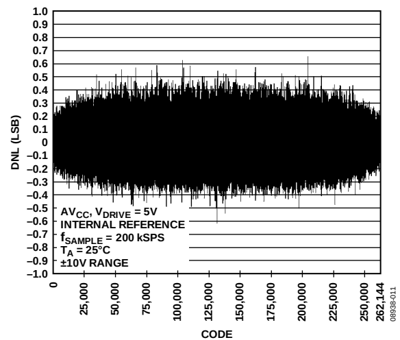
Figure 12. Typical DNL, \pm 10 \text{ V} Range
