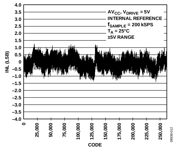
Figure 13. Typical INL, \pm 5 \text{ V} Range
