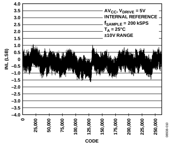
Figure 11. Typical INL, \pm 10 \text{ V} Range
