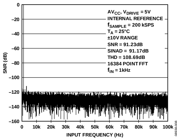
Figure 8. FFT Plot, \pm 10 \text{ V} Range
