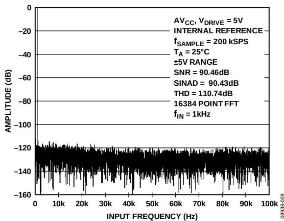
Figure 9. FFT Plot, \pm 5 \text{ V} Range
