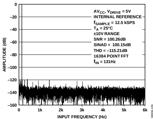
Figure 10. FFT Over Sampling by 16, \pm 10 \text{ V} Range
