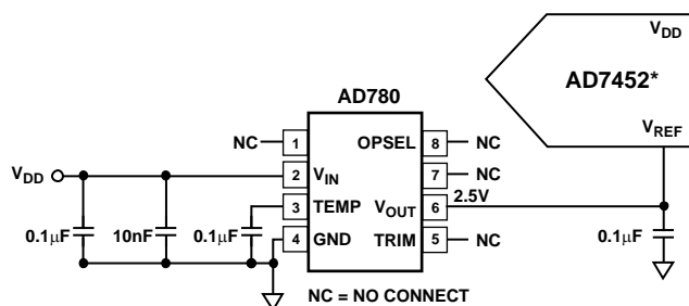
Figure 33. Typical V_{REF} Connection Diagram for V_{DD} = 5 V
