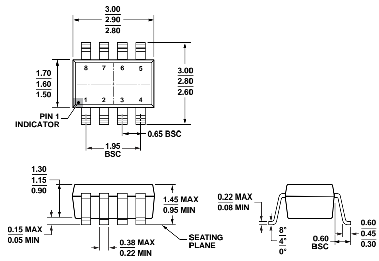
COMPLIANT TO JEDEC STANDARDS MO-178-BA Figure 40. 8-Lead Small Outline Transistor Package [SOT-23] (RJ-8) Dimensions shown in millimeters
