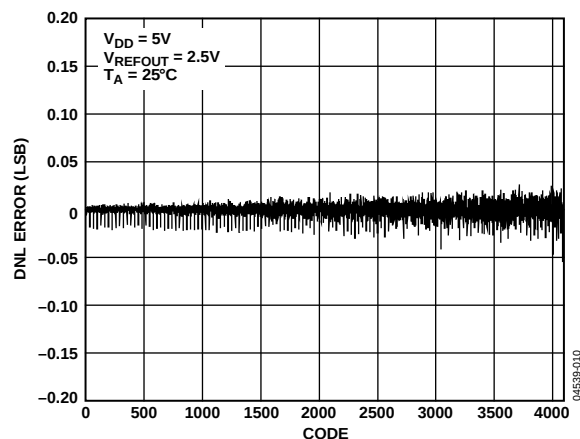
Figure 11. DNL—AD5620-2/AD6520-3
