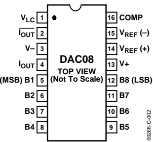
Figure 2. 16-Lead Dual In-Line Package (PDIP and Cerdip)
