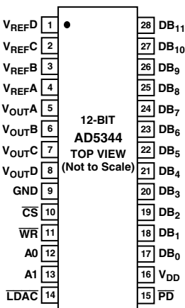
AD5344 PIN CONFIGURATION
