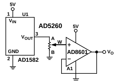
Figure 60. Programmable Voltage Reference
