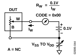
Figure 43. Incremental On Resistance
