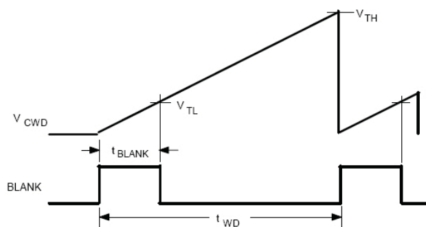
Watchdog-triggered commutation
