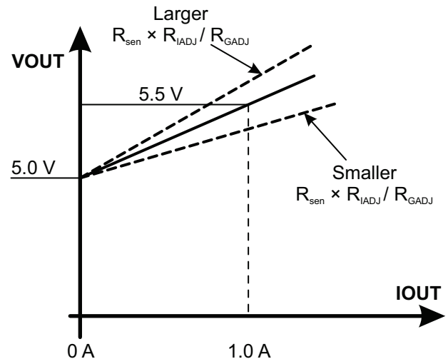
Figure 3: Voltage Correction Gain Adjustment
