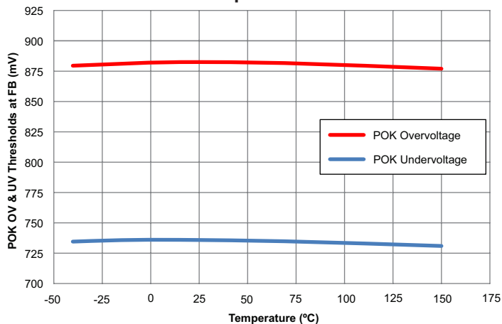
POK Overvoltage and Undervoltage Thresholds at FB versus Temperature (POK OV test with V_{GADJ} = 0 \text{ V} )
