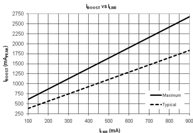
Figure 4. Boost inductor characteristic for the A8297.
