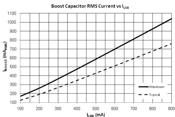
Figure 5. Boost electrolytic capacitor characteristic for the A8297.
