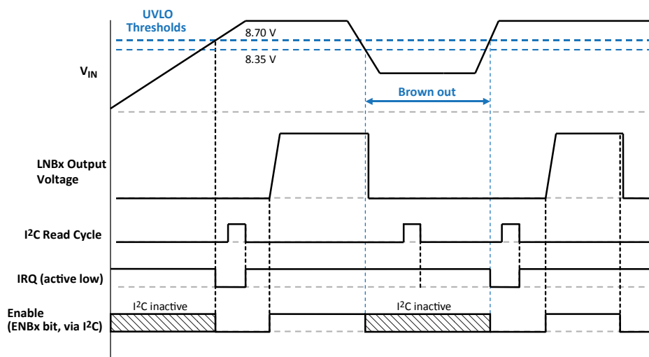
Figure 10. IRQ and Fault Clearing in Response to Undervoltage at V_{IN} (UVLO). At power-up, while V_{IN} is below 8.70 V (typ), the A8297 is disabled and the I 2 C port is inactive. After V_{IN} rises above 8.70 V (typ), the I 2 C port becomes active and the IRQ pin is pulled low. An I 2 C Read is required to report and clear the UVLO fault and set the IRQ pin to a logic high before the A8297 can be enabled. If a brown-out occurs, such that V_{IN} drops below 8.35 V (typ), the A8297 will be disabled and the I 2 C port will become inactive (note that the IRQ pin will remain high during this time because the A8297 is disabled). After V_{IN} rises above 8.70 V (typ) the I 2 C port reactivates and the IRQ pin is pulled low to report that a brown-out had occurred. An I 2 C Read is required to report and clear the UVLO fault before the A8297 can be re-enabled.
