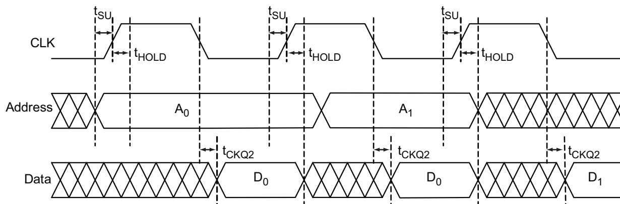
Figure 2-39 • Timing Diagram
