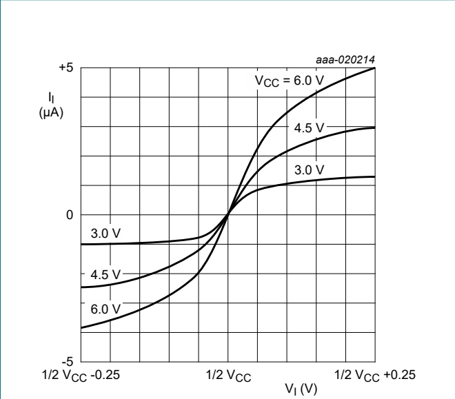
Fig. 15. Input current at SIG_IN, COMP_IN with \Delta V_I = 0.5\text{ V} at self-bias point
