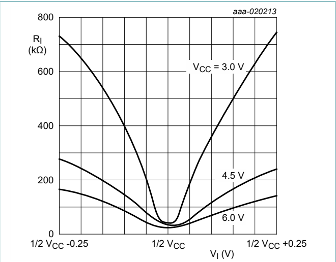
Fig. 14. Input resistance at SIG_IN, COMP_IN with \Delta V_I = 0.5\text{ V} at self-bias point
