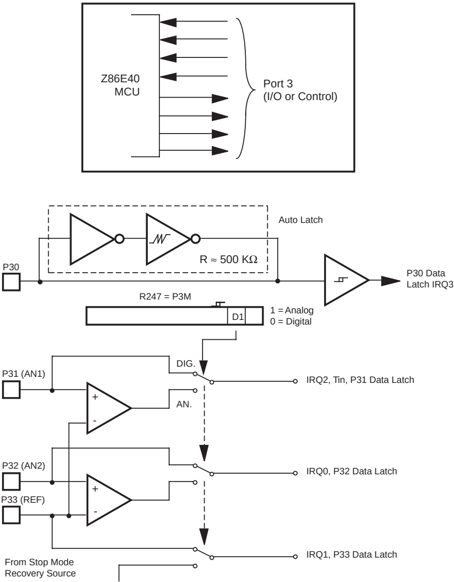
Figure 21. Port 3 Configuration
