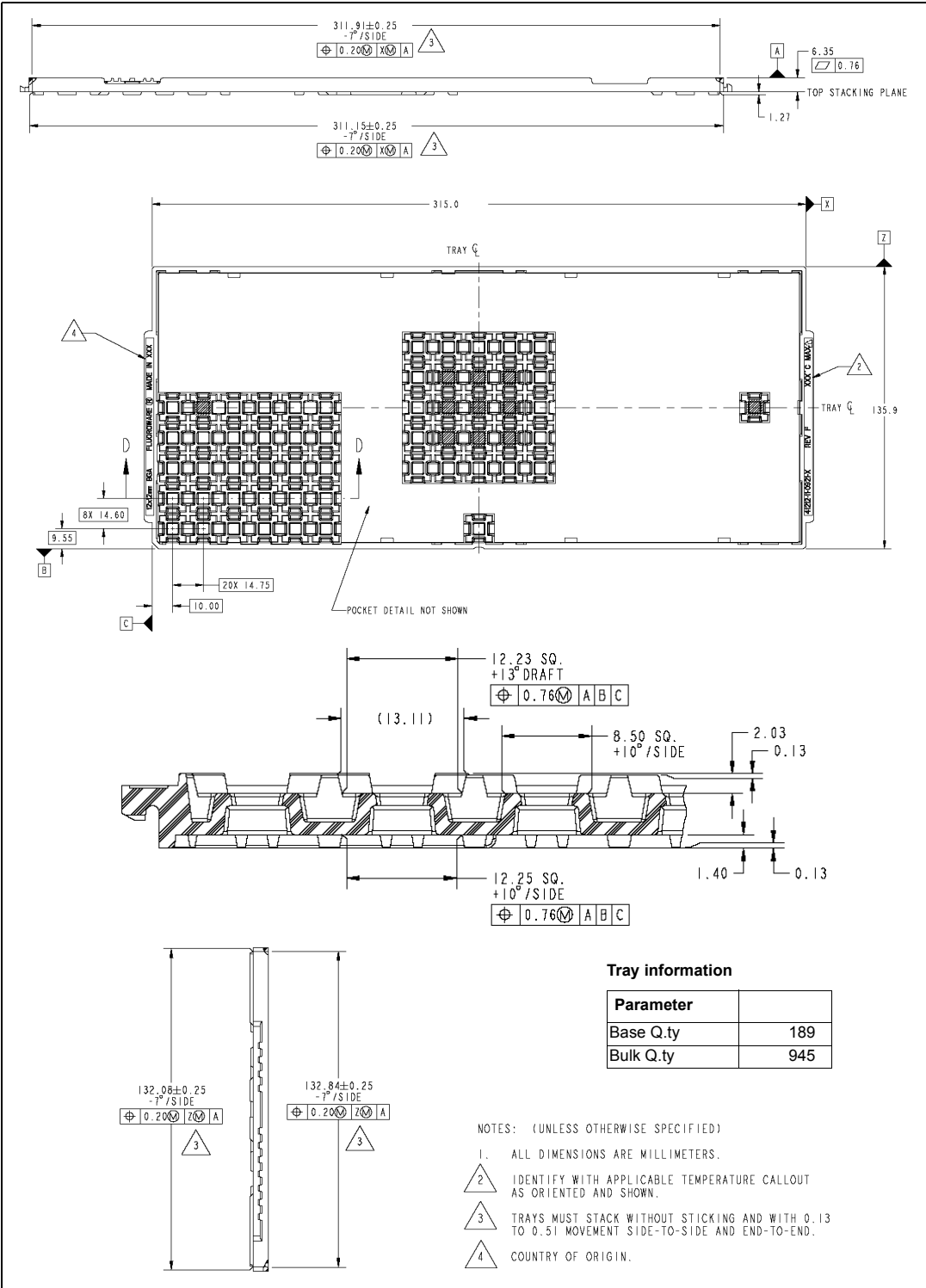
Figure 46. PQFN - 12x12 power lead-less tray shipment (no suffix)
