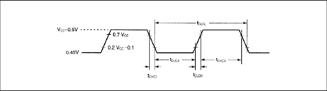
Figure 99. External clock cycle
