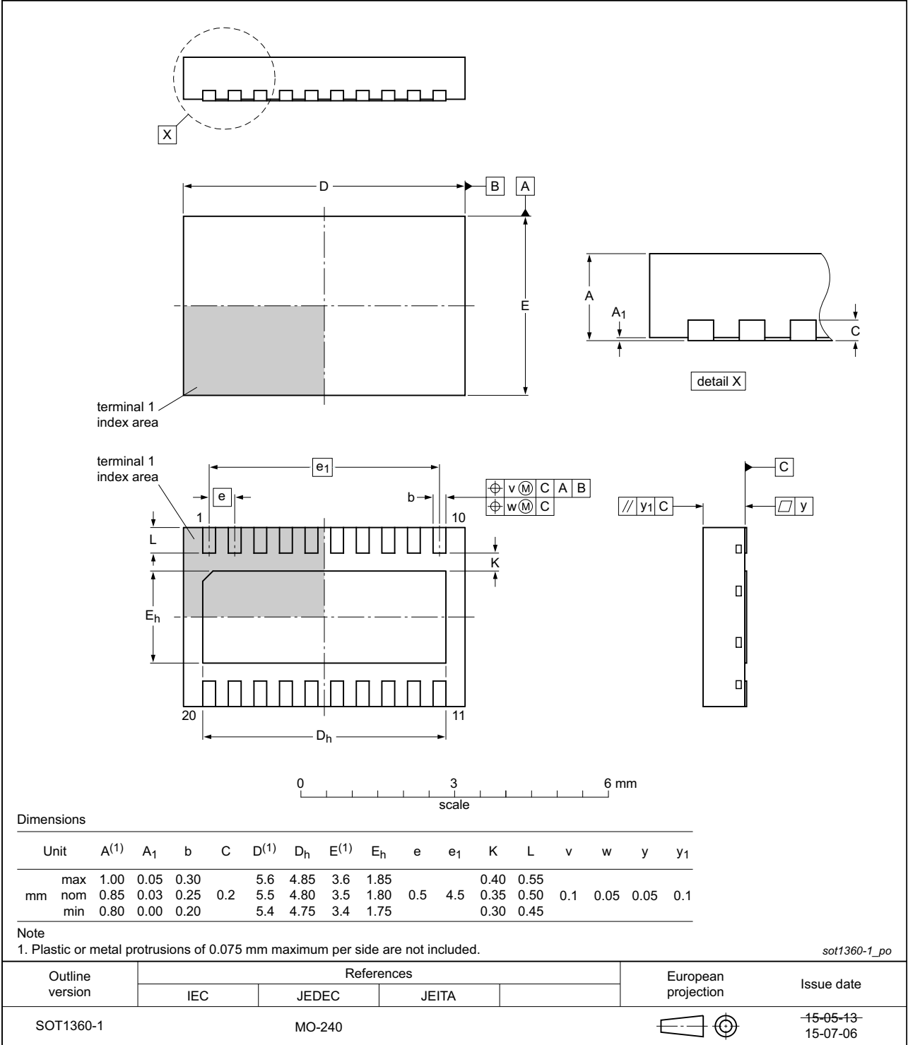
Fig 24. Package outline SOT1360-1 (HVSON20)
