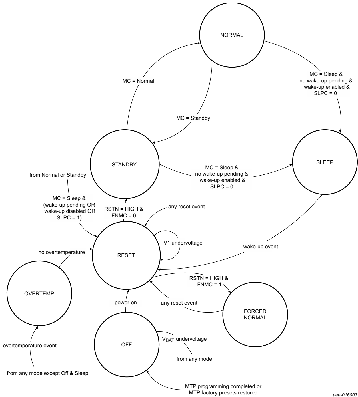
Fig 3. UJA1169A system controller state diagram
