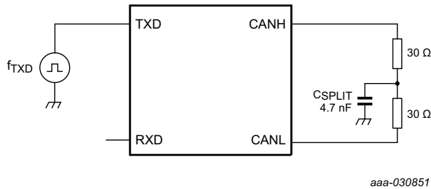
Fig 23. Test circuit for measuring transceiver driver symmetry
