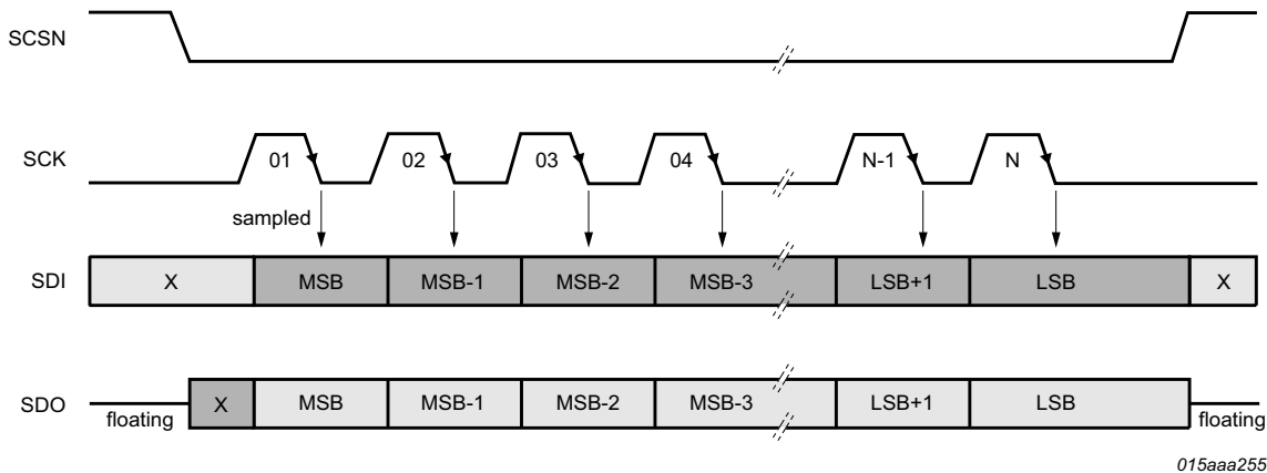
Fig 15. SPI timing overview (see Figure 20 for detailed SPI timing)
