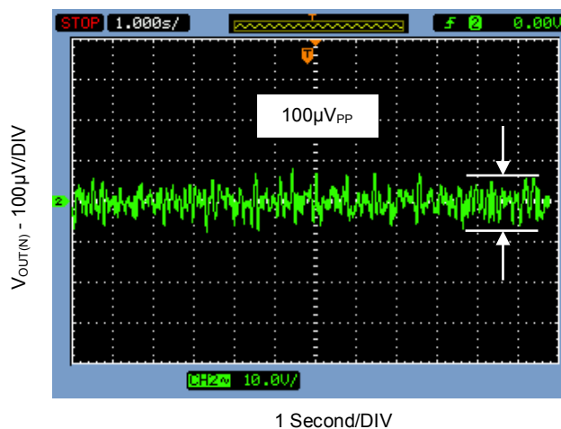
0.1Hz to 10Hz Output Voltage Noise
