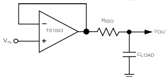
Figure 5: Using an External Resistor to Isolate a C_{LOAD} from the TS1003's Output
