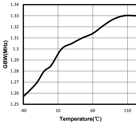
Unity Gain Bandwidth vs. Temperature
