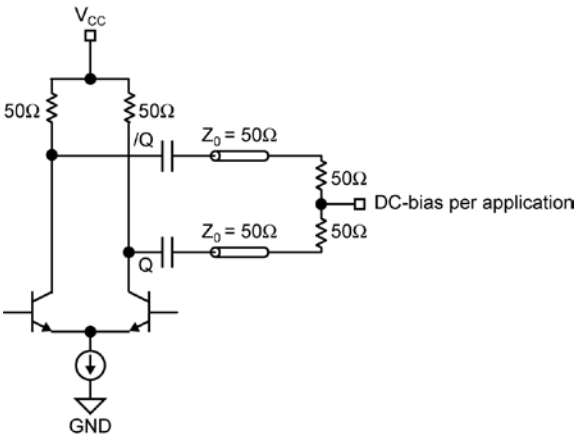
Figure 4c. CML AC-Coupled Termination
