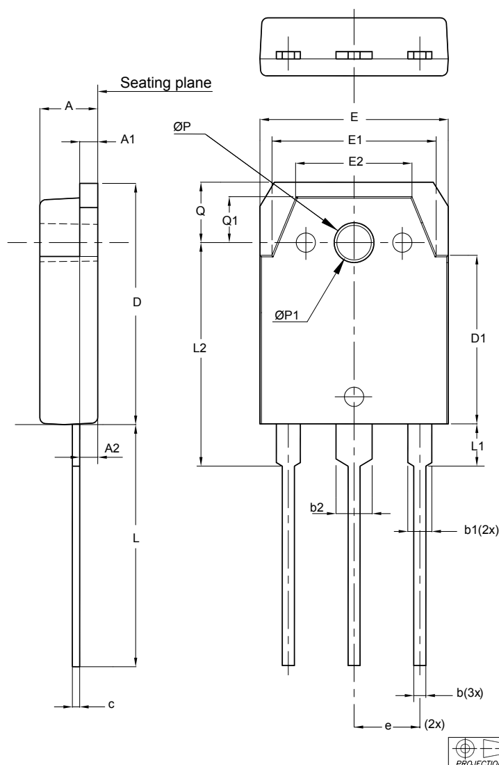
Figure 14. TO3P-3L package outline
