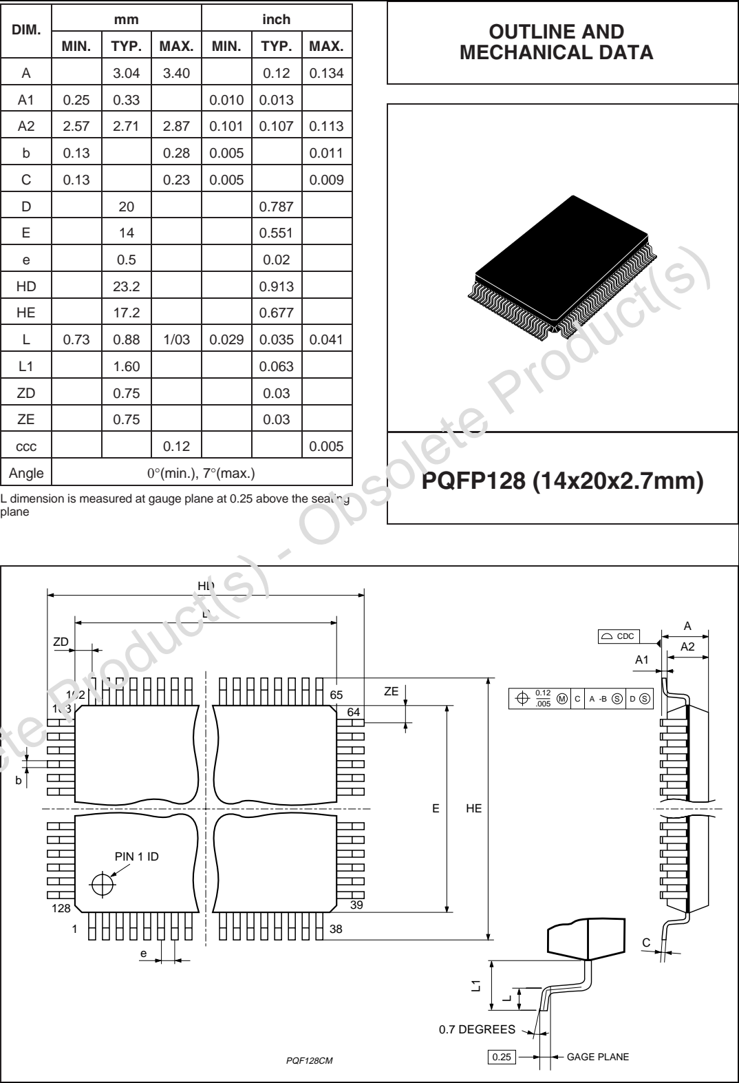
Figure 23. Package mechanical data
