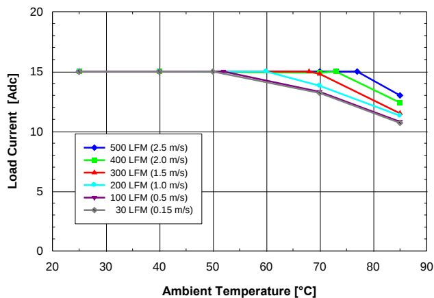
Fig. 3.3V.3: Available load current vs. ambient temperature and airflow rates for SQ24S15033 converter mounted vertically with V_{in} = 24V , air flowing from pin 3 to pin 1 and maximum FET temperature \leq 120^{\circ}C .
