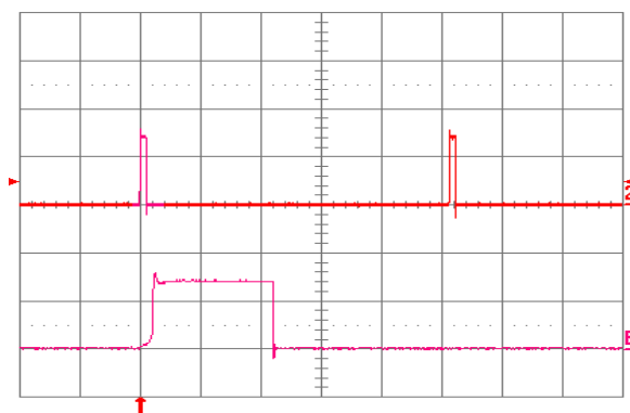
Fig. 5.0V.18: Load current (top trace, 10 A/div., 20 ms/div.) into a 10\ \text{m}\Omega short circuit during restart, at V_{in} = 24\ \text{V} . Bottom trace (10 A/div., 1 ms/div.) is an expansion of the on-time portion of the top trace.
