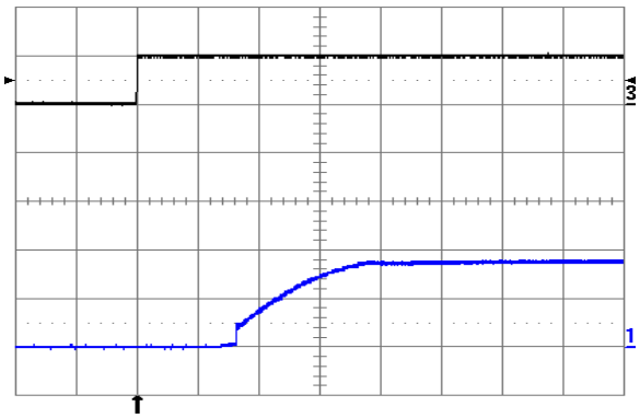
Fig. 1.8V.10: Turn-on transient at full rated load current (resistive) plus 10,000 µF at V_{in} = 24\text{V} , triggered via ON/OFF pin. Top trace: ON/OFF signal (5 V/div.). Bottom trace: output voltage (1 V/div.). Time scale: 1 ms/div.
