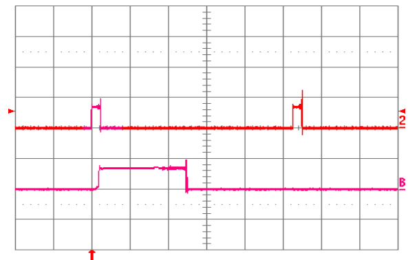
Fig. 6.0V.18: Load current (top trace, 20\ \text{A}/\text{div} ., 20\ \text{ms}/\text{div} .) into a 10\ \text{m}\Omega short circuit during restart, at V_{in} = 24\ \text{V} . Bottom trace ( 20\ \text{A}/\text{div} ., 2\ \text{ms}/\text{div} .) is an expansion of the on-time portion of the top trace.
