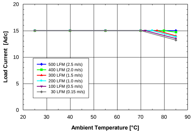
Fig. 2.0V.3: Available load current vs. ambient temperature and airflow rates for SQ24S15020 converter mounted vertically with V_{in} = 24V , air flowing from pin 3 to pin 1 and maximum FET temperature \leq 120^{\circ}C .
