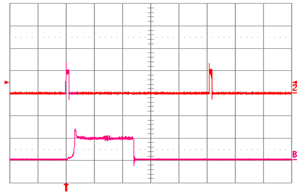
Fig. 2.5V.18: Load current (top trace, 20\ \text{A}/\text{div.} , 20\ \text{ms}/\text{div.} ) into a 10\ \text{m}\Omega short circuit during restart, at V_{in} = 24\ \text{V} . Bottom trace ( 20\ \text{A}/\text{div.} , 1\ \text{ms}/\text{div.} ) is an expansion of the on-time portion of the top trace.
