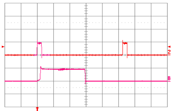
Fig. 1.8V.18: Load current (top trace, 20\ \text{A}/\text{div} ., 20\ \text{ms}/\text{div} .) into a 10\ \text{m}\Omega short circuit during restart, at V_{in} = 24\ \text{V} . Bottom trace ( 20\ \text{A}/\text{div} ., 2\ \text{ms}/\text{div} .) is an expansion of the on-time portion of the top trace.
