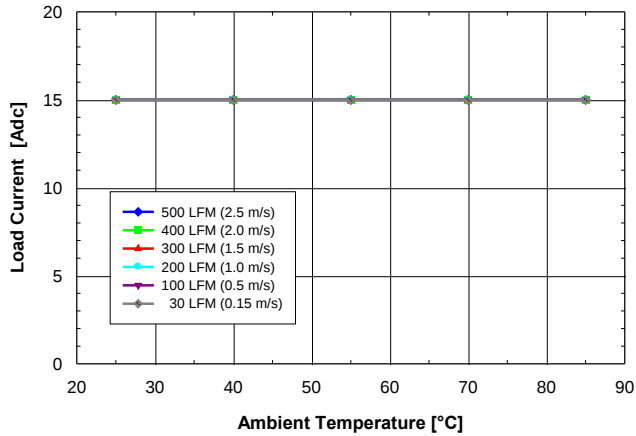
Fig. 1.0V.3: Available load current vs. ambient temperature and airflow rates for SQ24S15010 converter mounted vertically with V_{in} = 24V , air flowing from pin 3 to pin 1 and maximum FET temperature \leq 120^{\circ}C .
