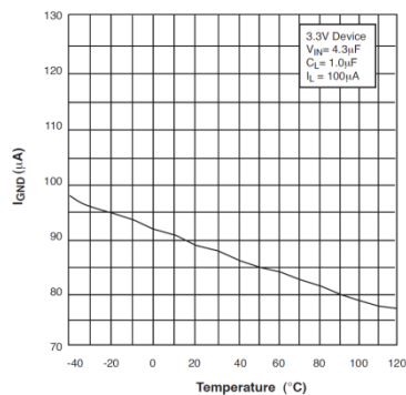
Fig. 9 Ground Current vs Temperature with 100 \mu A Load
