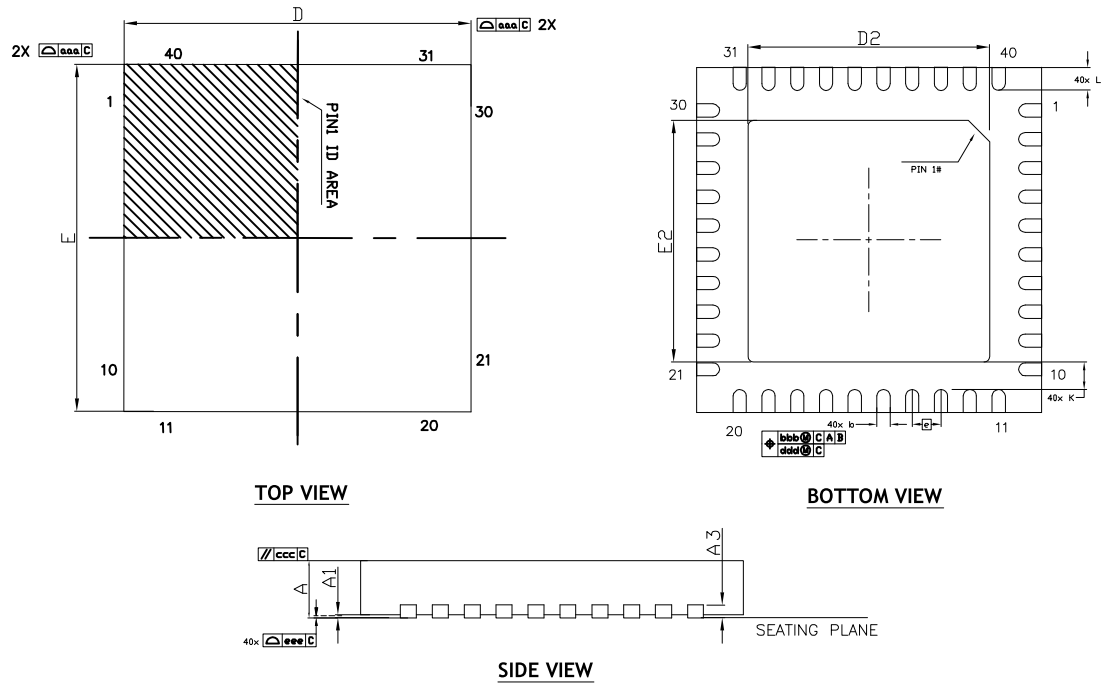
FIGURE 19. QFN40
