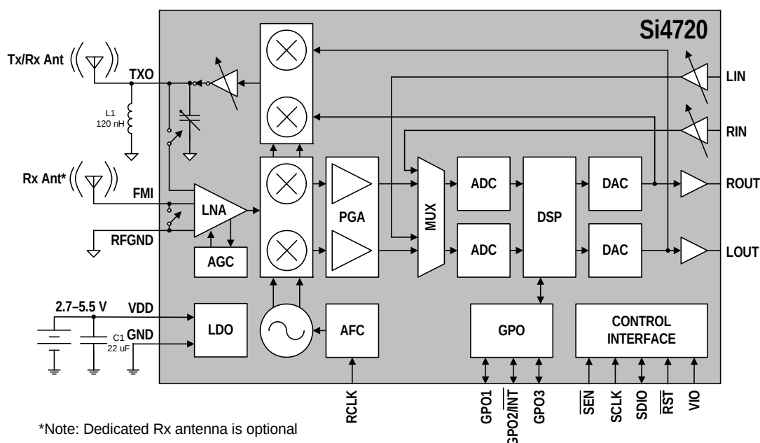
Figure 14. Functional Block Diagram
