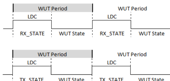
Figure 27.1. RX and TX LDC Sequences
