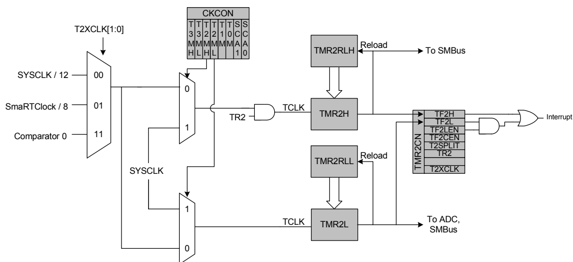
Figure 31.5. Timer 2 8-Bit Mode Block Diagram
