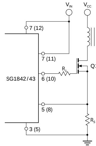
FIGURE 16. — MOSFET PARASITIC OSCILLATIONS
