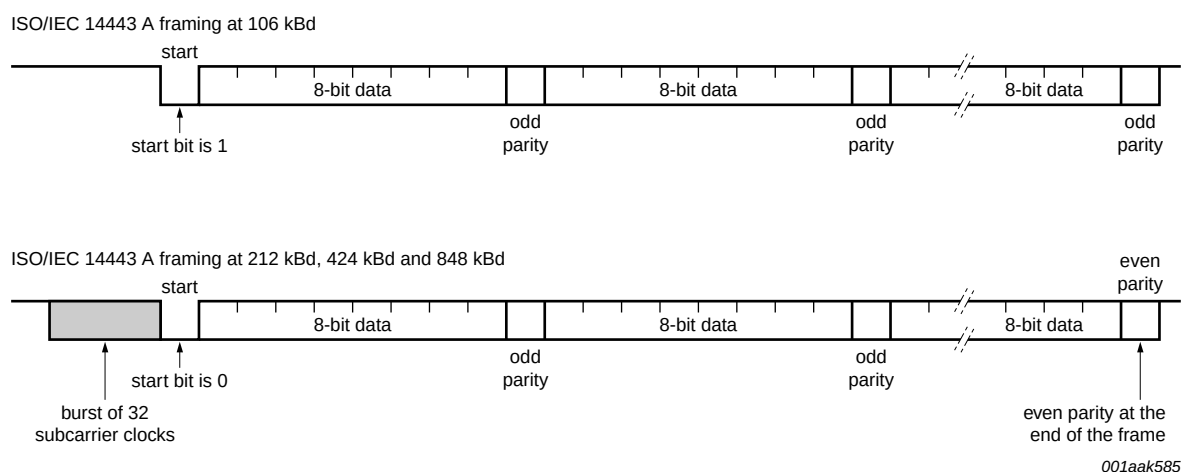
Fig 20. Data coding and framing according to ISO/IEC 14443 A card response
