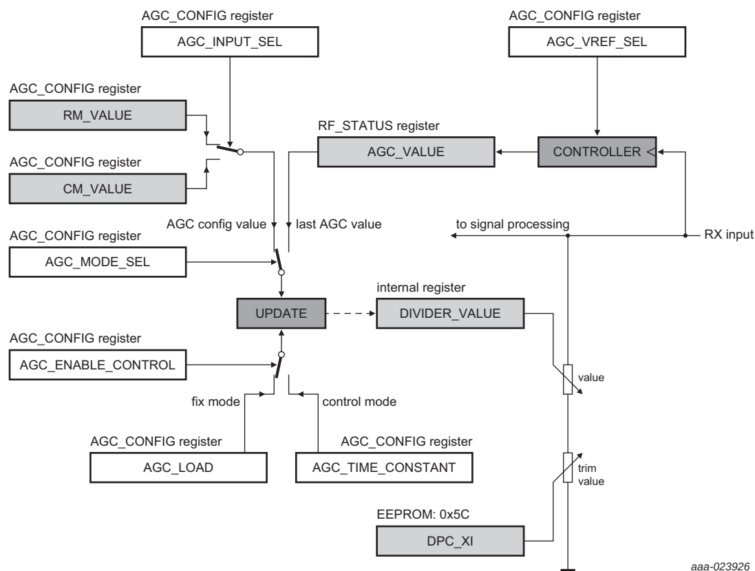
Fig 35. DPC, AGC and AWC configuration
