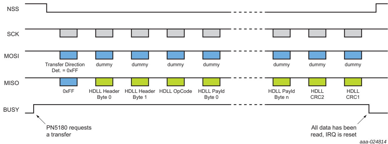
Fig 43. Secure Firmware Download: SPI Read
