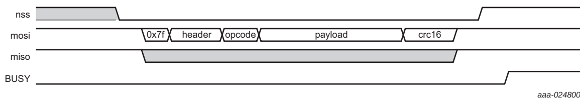
Fig 40. Example SPI WRITE in Secure Firmware Download mode
