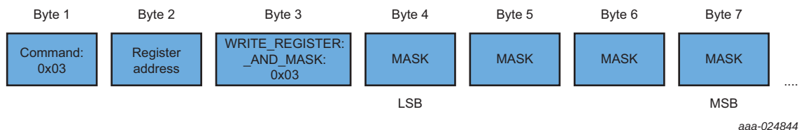
Fig 14. WRITE REGISTER AND MASK
