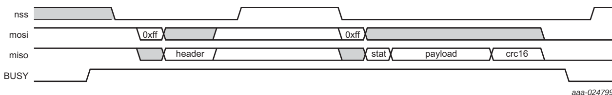
Fig 41. Example SPI READ in Secure Firmware Download mode
