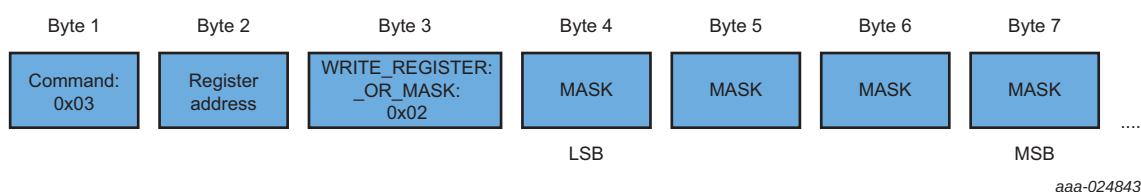
Fig 13. WRITE REGISTER OR MASK
