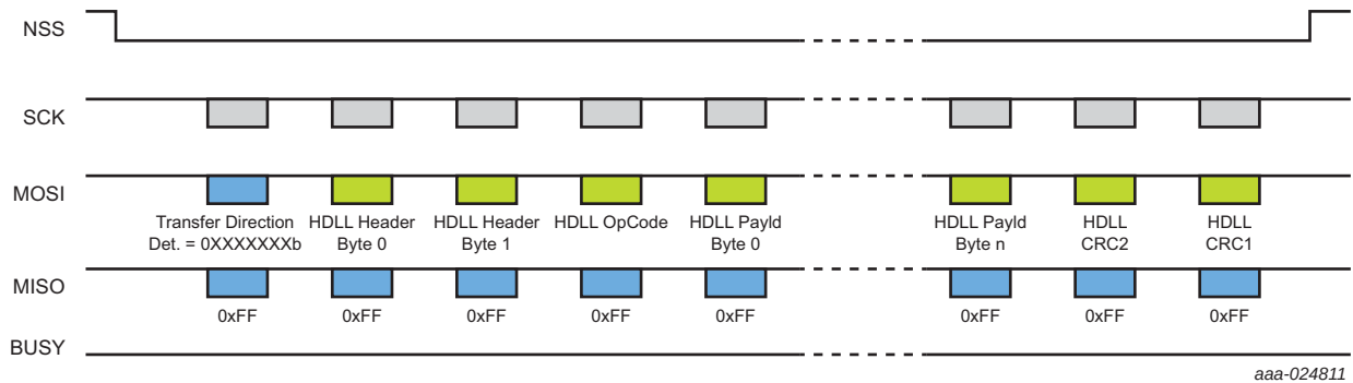
Fig 42. Secure Firmware Download: SPI Write
