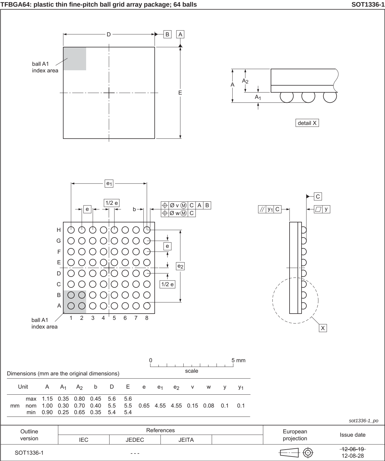
Fig 53. Package outline package version (TFBGA64)
