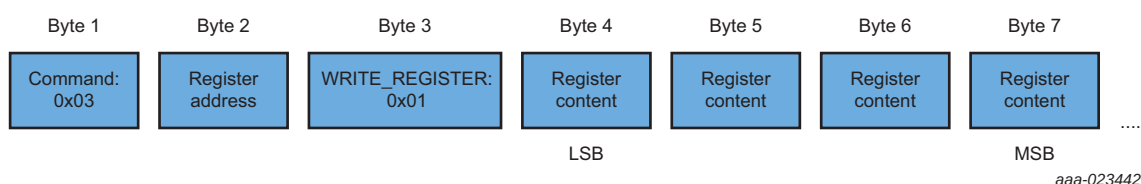
Fig 12. Write_Register_Multiple
