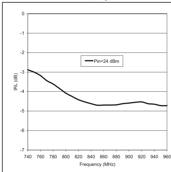
Figure 5. Input return loss vs frequency Vdd = 7.2 V, Idq = 200 mA
