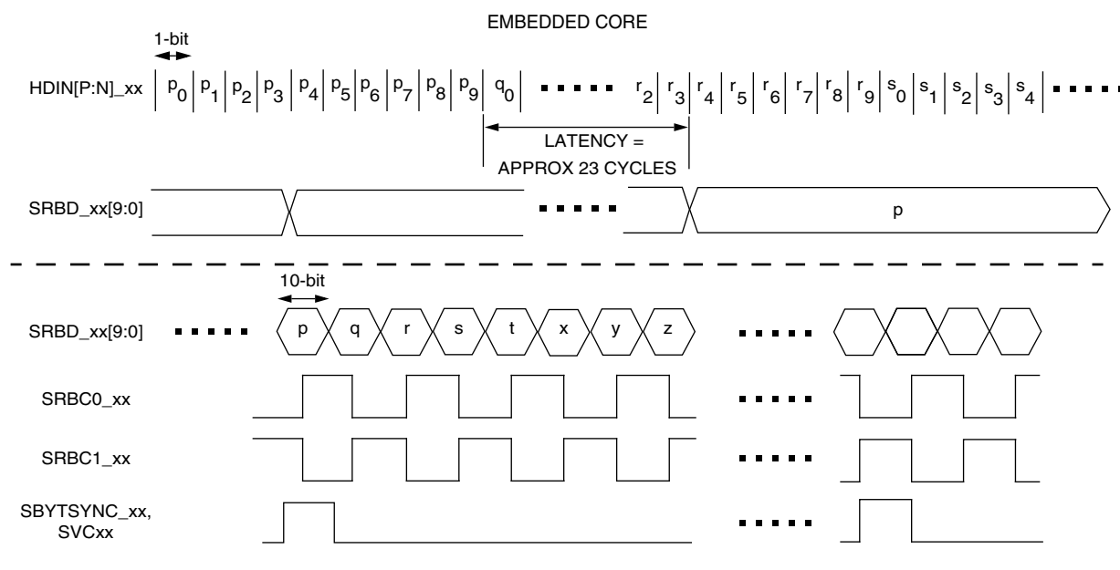
Figure 7. Receive Path Timing for a Single SERDES Channel
