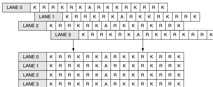
Figure 16. Deskew Lanes by Aligning /A/ Columns
