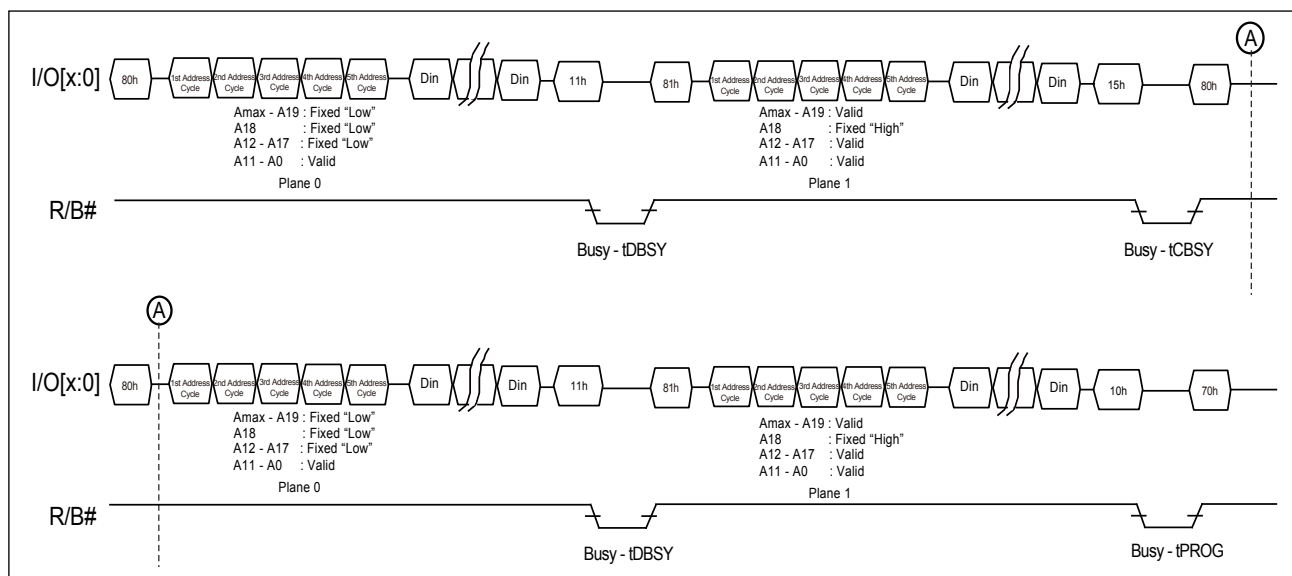
Figure 39. AC waveforms for Two-plane Cache Program (Traditional)
