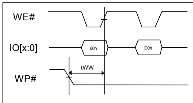
Figure 46-4. Disable Erasing of WP# Signal
