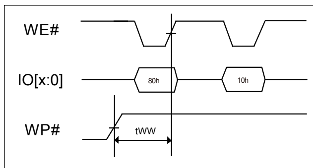
Figure 46-1. Enable Programming of WP# Signal
