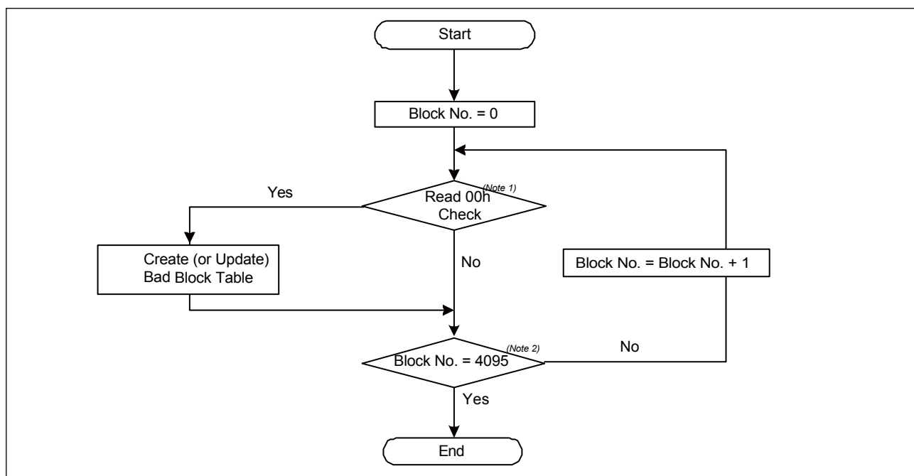
Figure 48. Bad Block Test Flow
