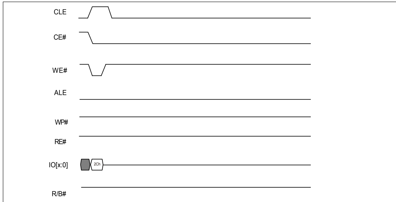
Figure 40. AC Waveforms for Block Solid-Protect
