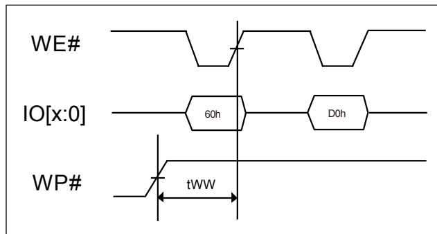
Figure 46-3. Enable Erasing of WP# Signal
